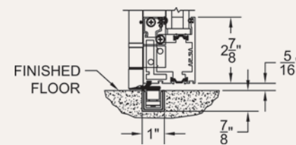
Optional: Flush Sill Guide Sill
