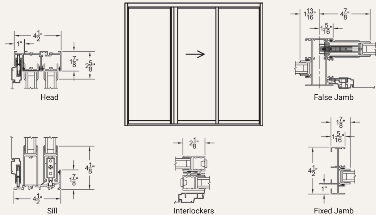
Elevation View: OXOL Configuration
