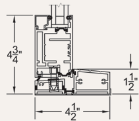
Sill (Outswing)
