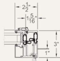
Nail-On Jamb at Hinge
