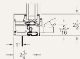
Nail-On Sill Casement
