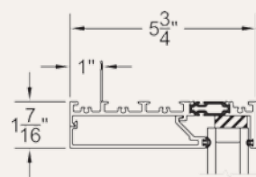
Nail-On Head
