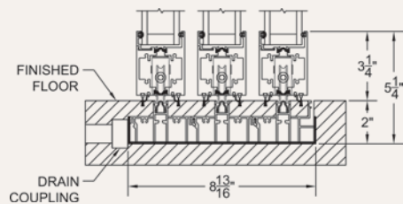
Sill
