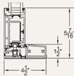
Sill
