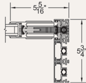
Lock Jamb-Right
