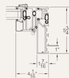
Nail-On Jamb with 450-T Insert
