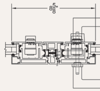
Meetings Stiles (Integral Hinged Door)
