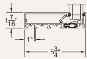
Nail-On Sill
